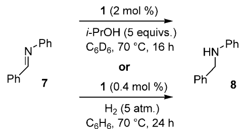
Scheme 6. Imine reduction by transfer hydrogenation with 2-propanol and direct hydrogenation.
