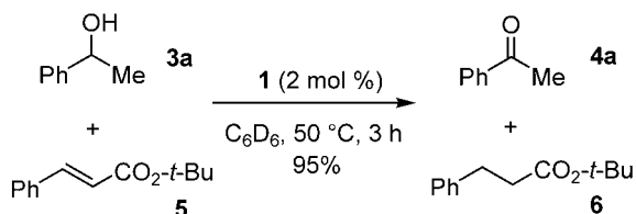
Scheme 5. Crossover transfer hydrogenation.
