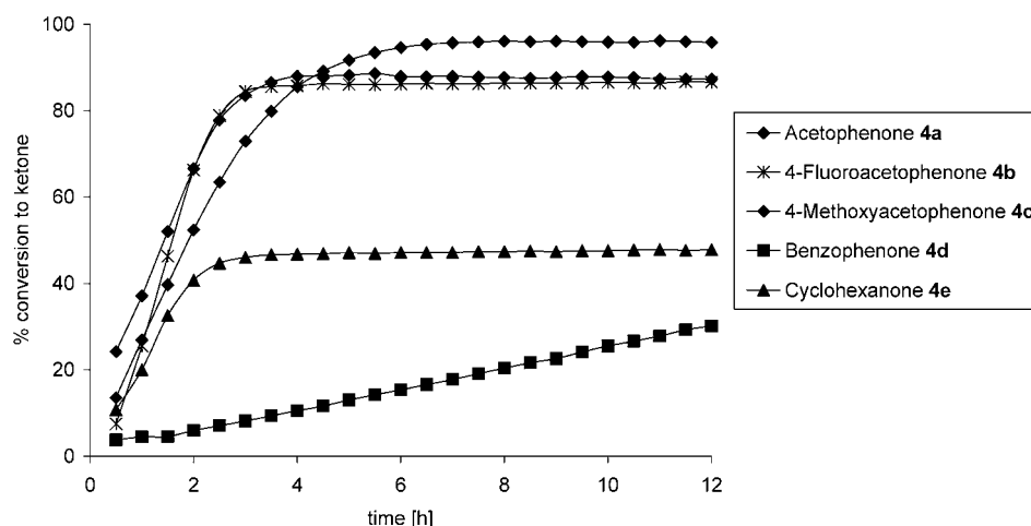
Figure 1. Oxidation of alcohols 3a–e to ketones 4a–e by transfer hydrogenation with acetone (5 equivs.) catalysed by complex 1 (2 mol %). Reactions were monitored by 1 H NMR and conversions are based on integration of the 1 H signals.
