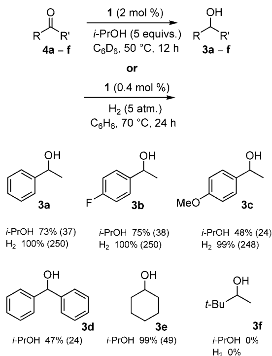
Scheme 4. Ketone reduction by transfer hydrogenation with 2-propanol and direct hydrogenation. Numbers in brackets are turnover numbers (TON).
