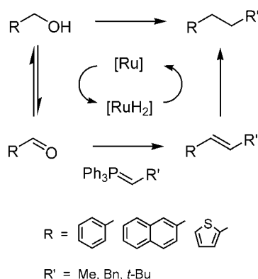
Scheme 1. Indirect Wittig reaction of alcohols.
