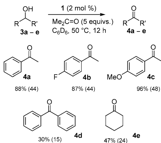
Scheme 3. Alcohol oxidation by transfer hydrogenation with acetone. Numbers in brackets are turnover numbers (TON).
