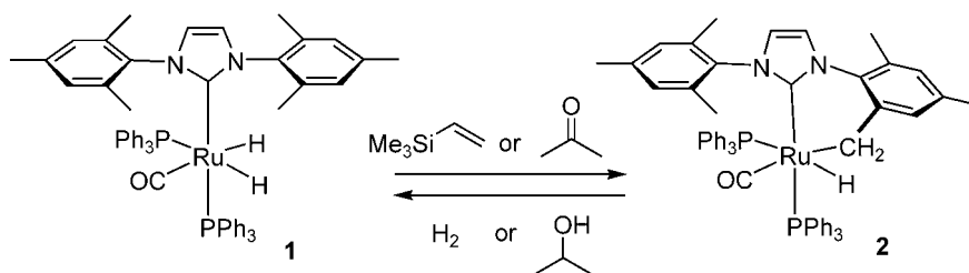
Scheme 2. Reversible dehydrogenation/hydrogenation of complex 1 .
